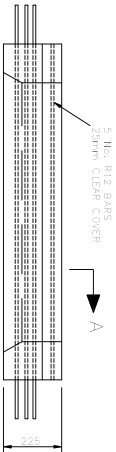
PLAN
