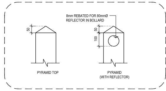
3 BOLLARD TOP FORM ELEVATION SCALE: NTS
