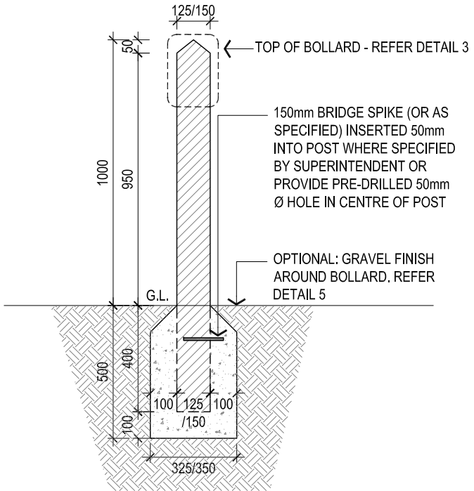
2 BOLLARD DETAIL SECTION SCALE 1:20
