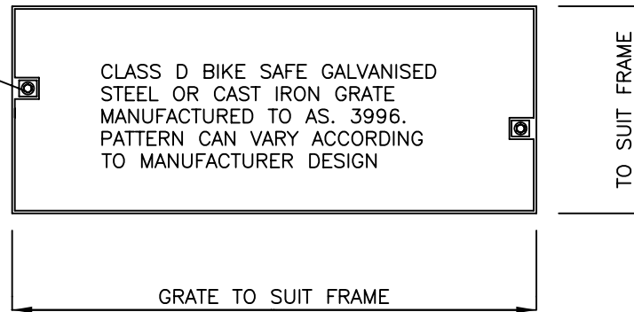
GRATE
