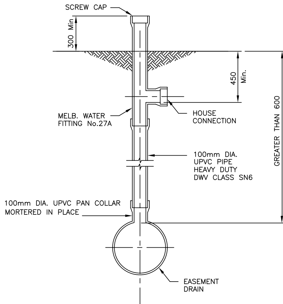
TYPE 'A' DEEP CONNECTION
