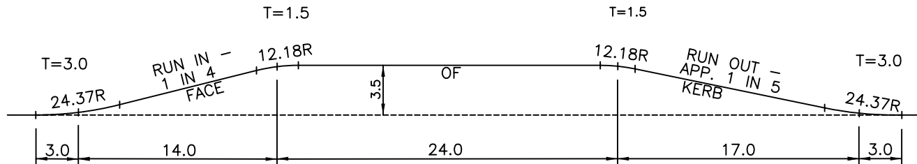
INDENTED STORAGE BAY FOR TWO BUSES
