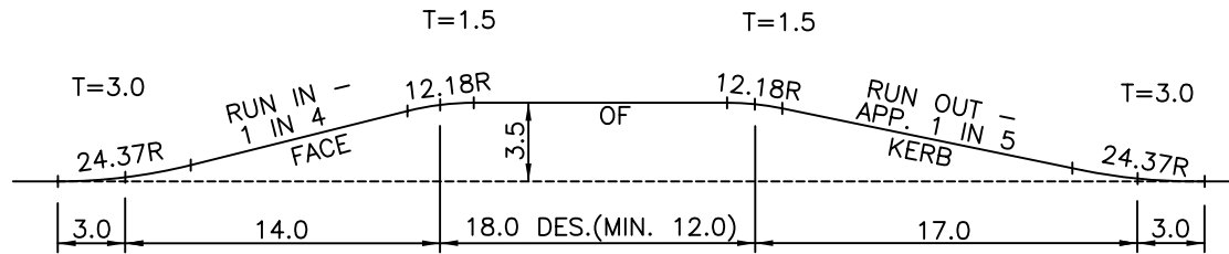
INDENTED STORAGE BAY FOR ONE BUS
