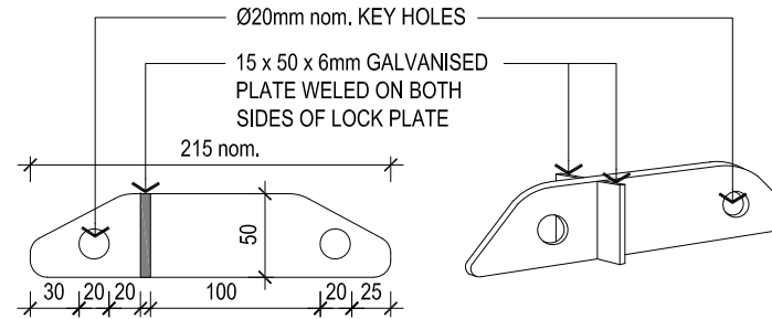
2 DOUBLE LOCK PLATE ELEVATION AND 3D VIEW SCALE 1:5
