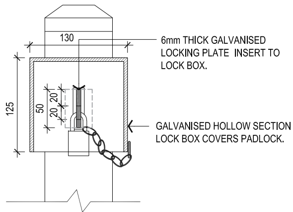
3 LOCK BOX FRONT SECTION SCALE 1:5
