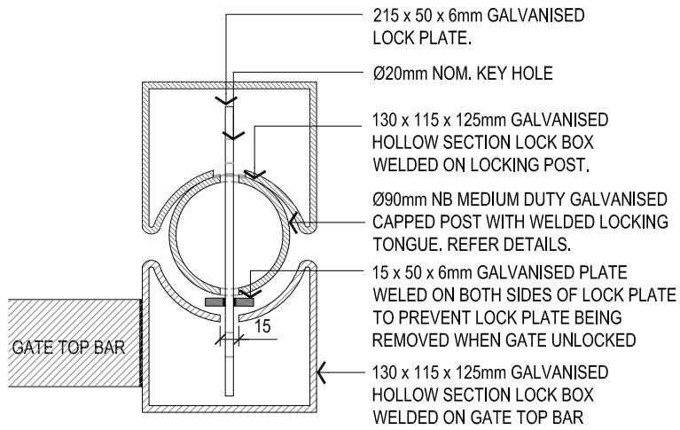
1 DOUBLE LOCK BOX PLAN SCALE 1:5
