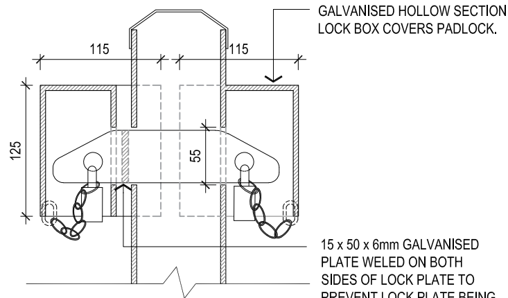
4 DOUBLE LOCK BOX SIDE SECTIONS SCALE 1:5
